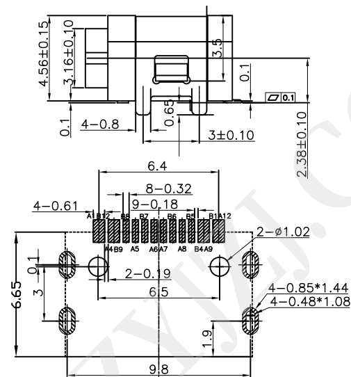
RECOMMENDED PCB LAYOUT Tolerance: ±0.05mm
